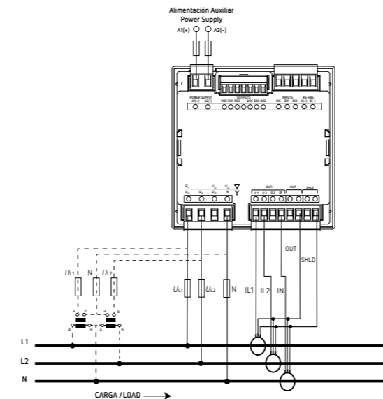
Red bifásica a 3 hilos / 3-wire two-phase network
