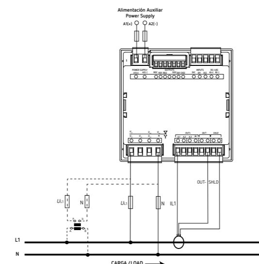
Red monofásica fase-neutro de 2 hilos 2-wire Single-phase network (Neutral)
